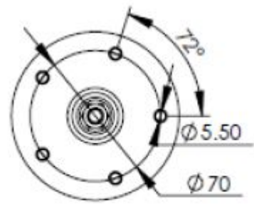
Relevant mounting dimensions on part
