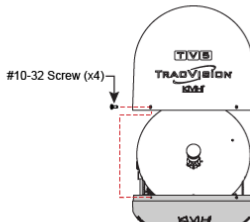
Figure 4-1 Radome Removal
