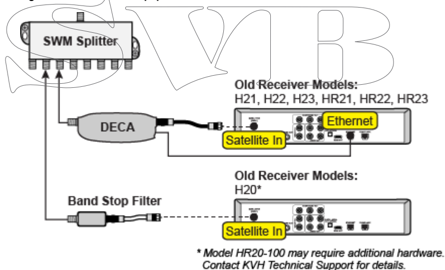
Figure 7-5 Additional Equipment for Older Receivers
