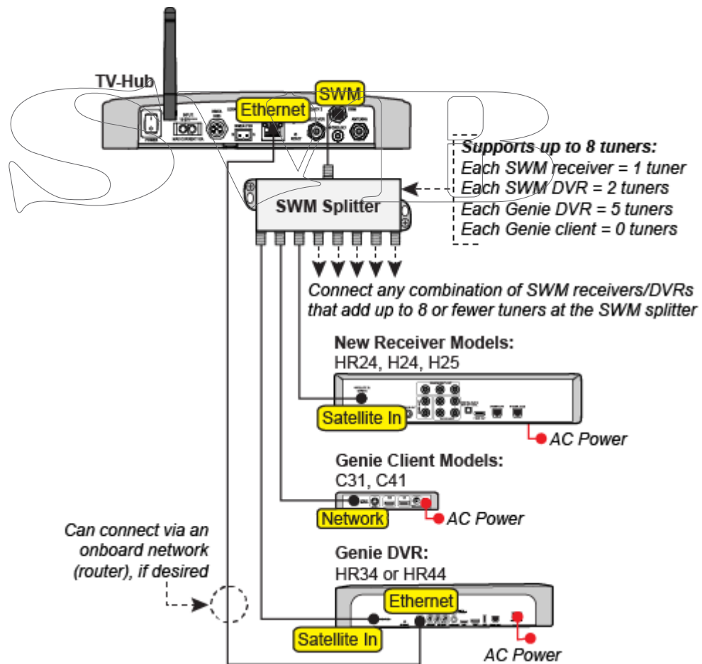
Figure 7-4 Genie Configuration
