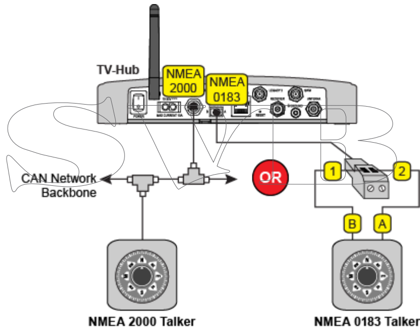
Figure 4-4 TV-Hub NMEA Connections (TV-Hub A shown)
