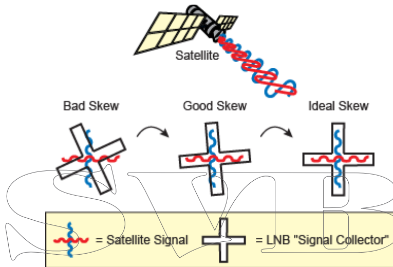
Figure 4-3 How Skew Works
