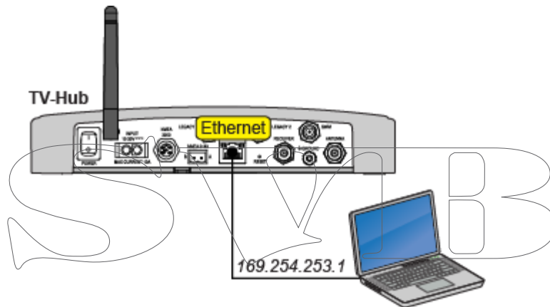
Figure 3-5 TV-Hub Direct Wired Connection (TV-Hub A shown)
