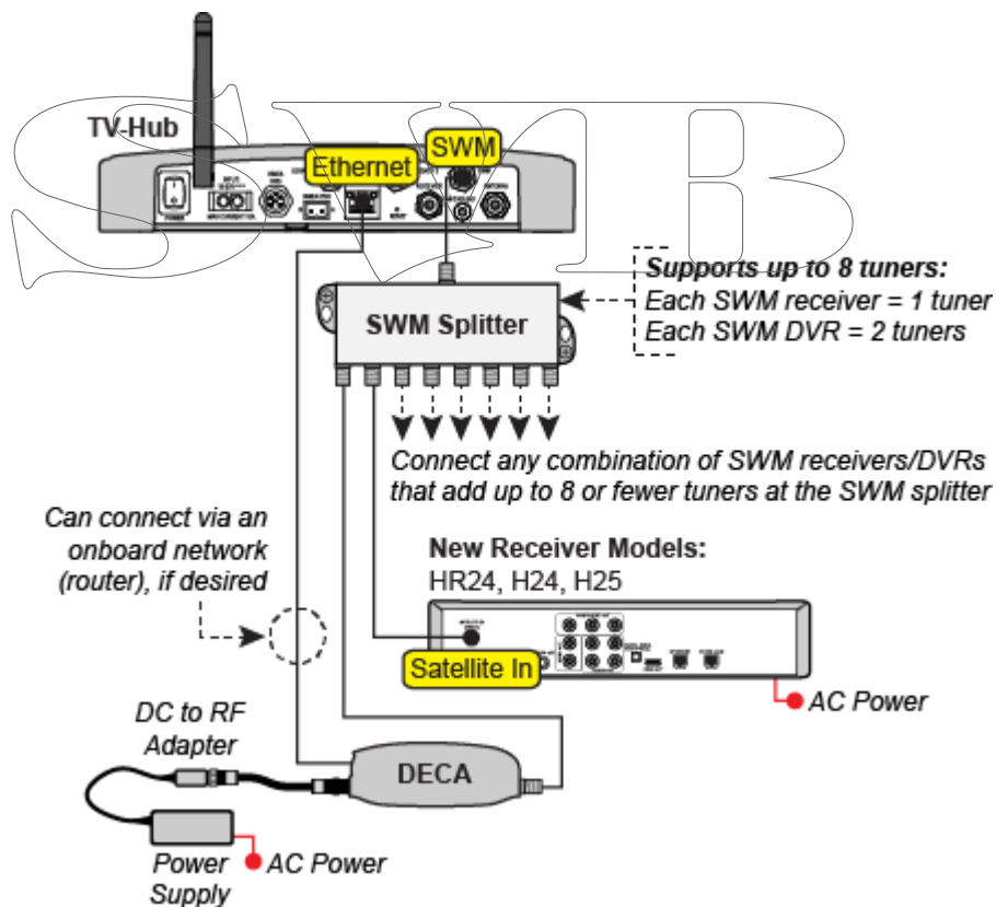
Figure 7-3 Non-Genie Configuration
