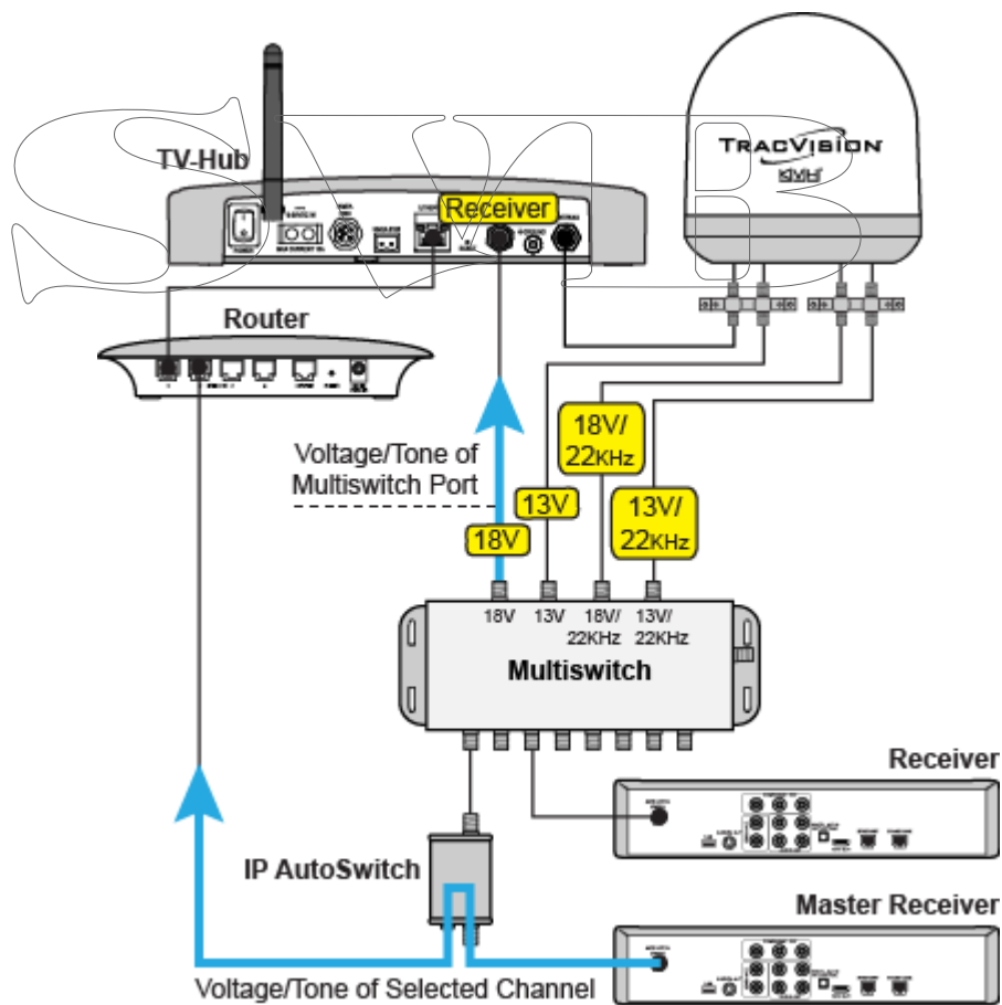
Figure 4-5 Example of Conflicting Band/Polarization Requests
