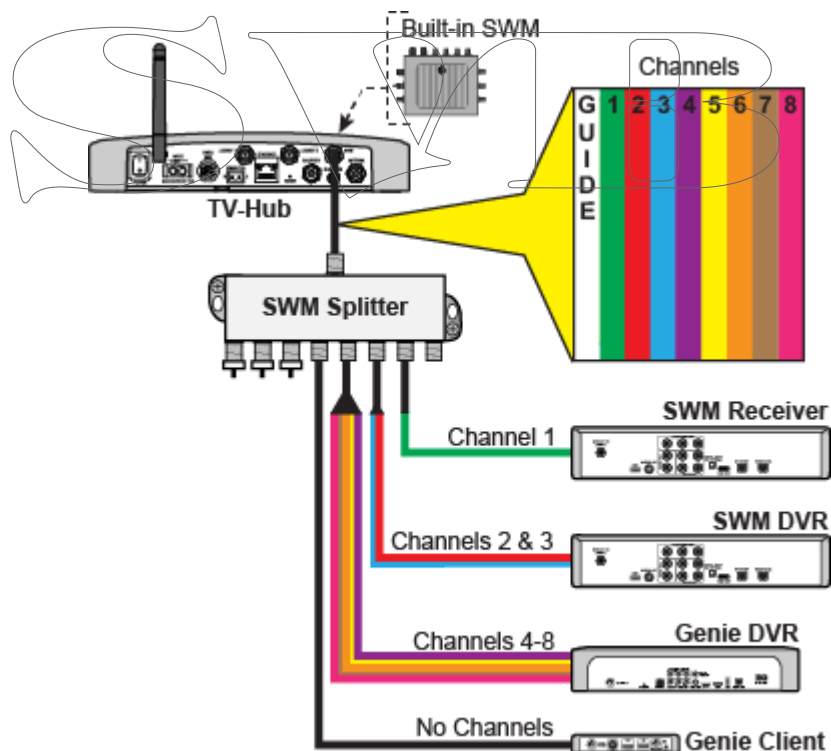
Figure 7-7 DIRECTV SWM Technology
