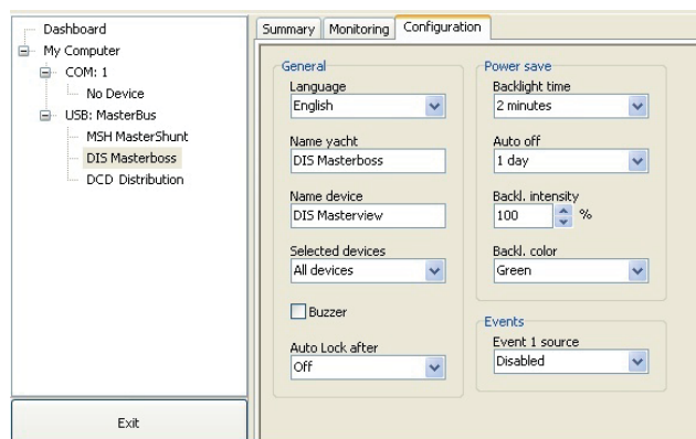
Figura 13: software MasterAdjust
