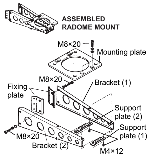
How to assemble the radome mount
