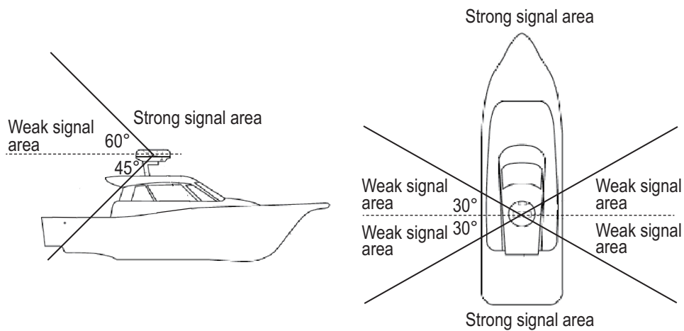
Location and wireless LAN communication range
